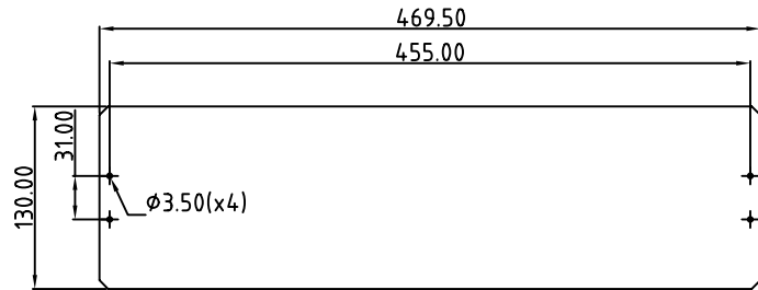
Anodised Front Panel 2mm Thick
