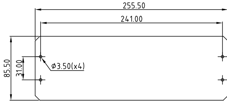
Anodised Front Panel 2mm Thick
